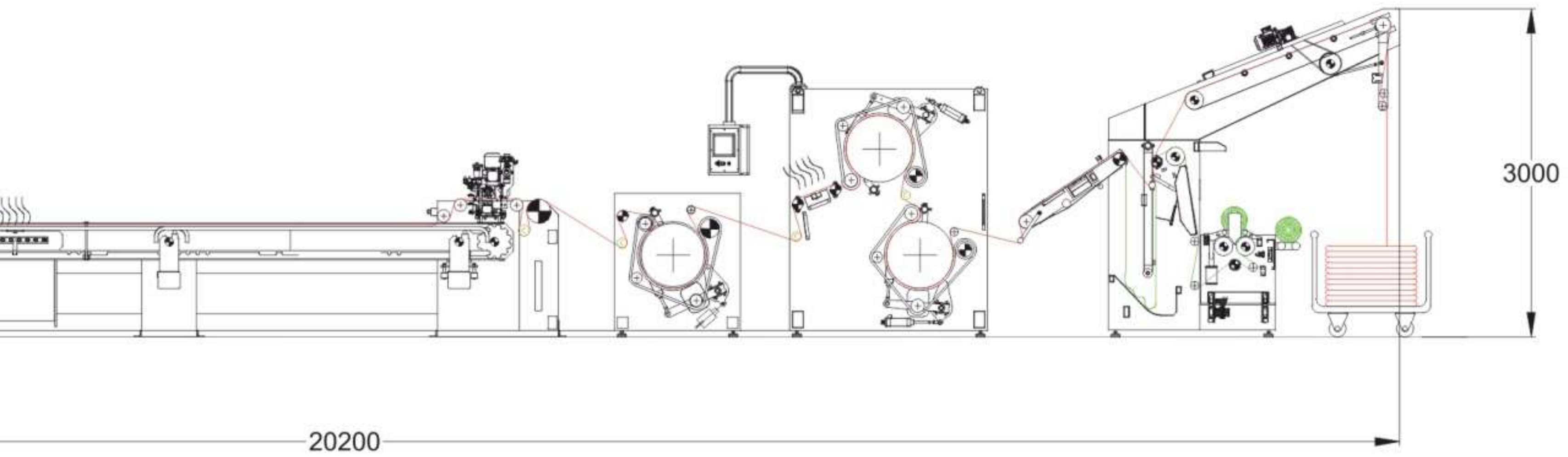
Felt Compactor with Pin Chain Tenter Frame + Shrink F3 Egalizeli Açık En Keçeli Sanfor + Shrink F3
