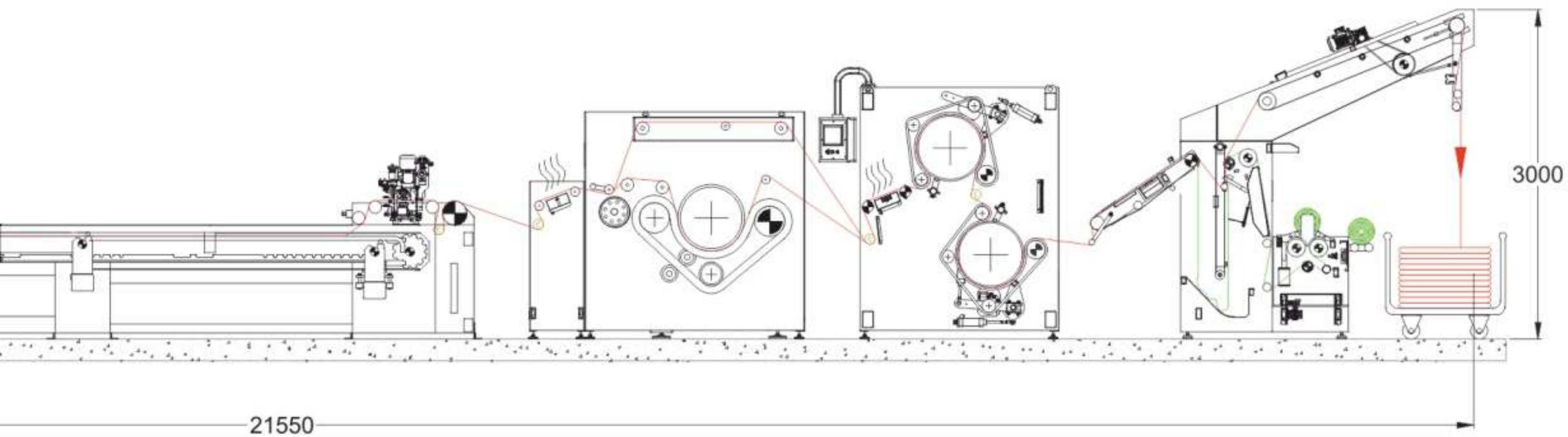
Felt Compactor with Pin Chain Tenter Frame + Rubber Egalizeli Açık En Keçeli Sanfor + Kauçuk Blanket
