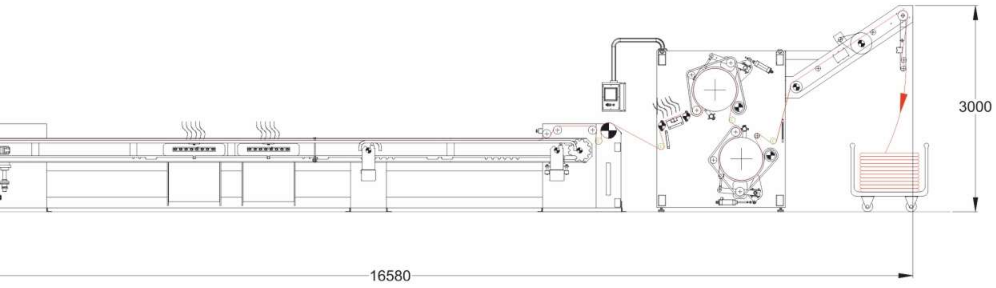
Felt Compactor with Pin Chain Tenter Frame (Standard) Egalizeli Açık En Keçeli Sanfor (Standart)
