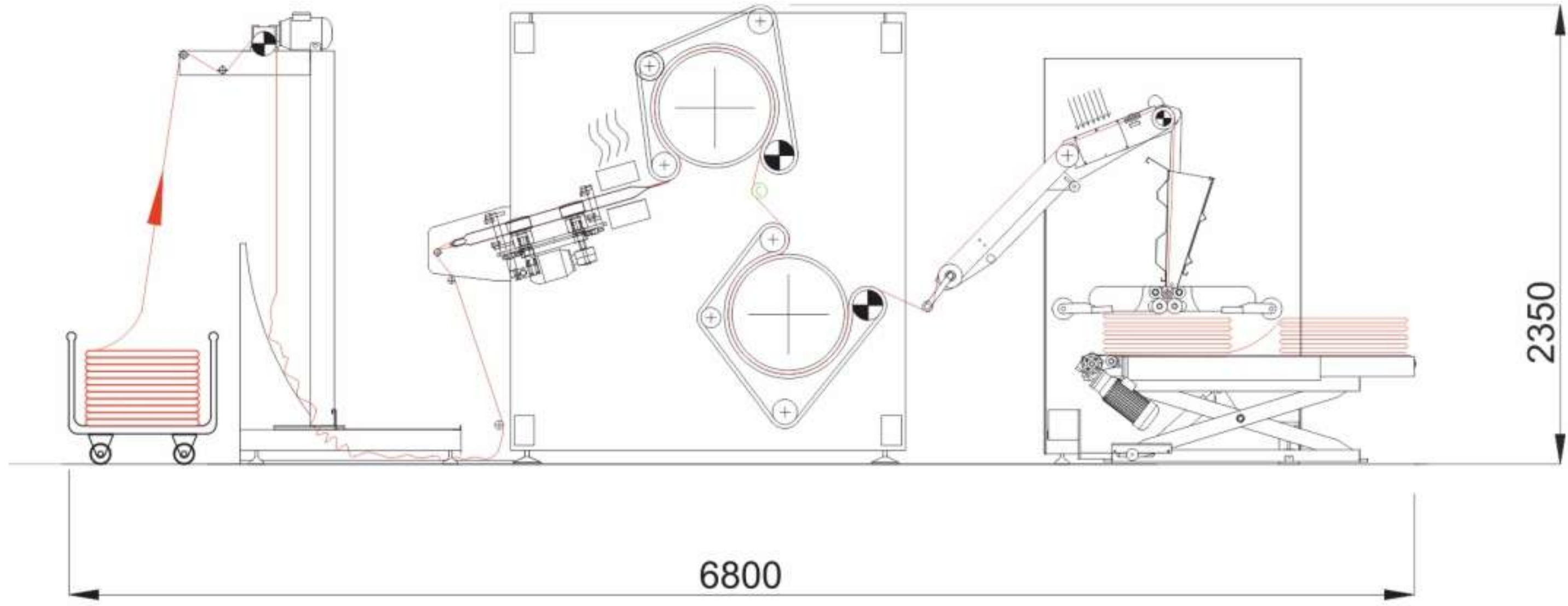
Tubular Felt Compactor Tüp Keçeli Sanfor
