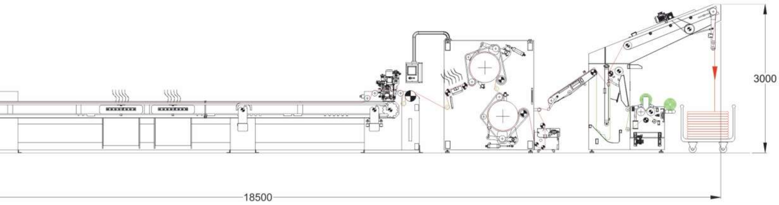
Felt Compactor with Pin Chain Tenter Frame (Full Option) Egalizeli Açık En Keçeli Sanfor (Tam Opsiyon)
